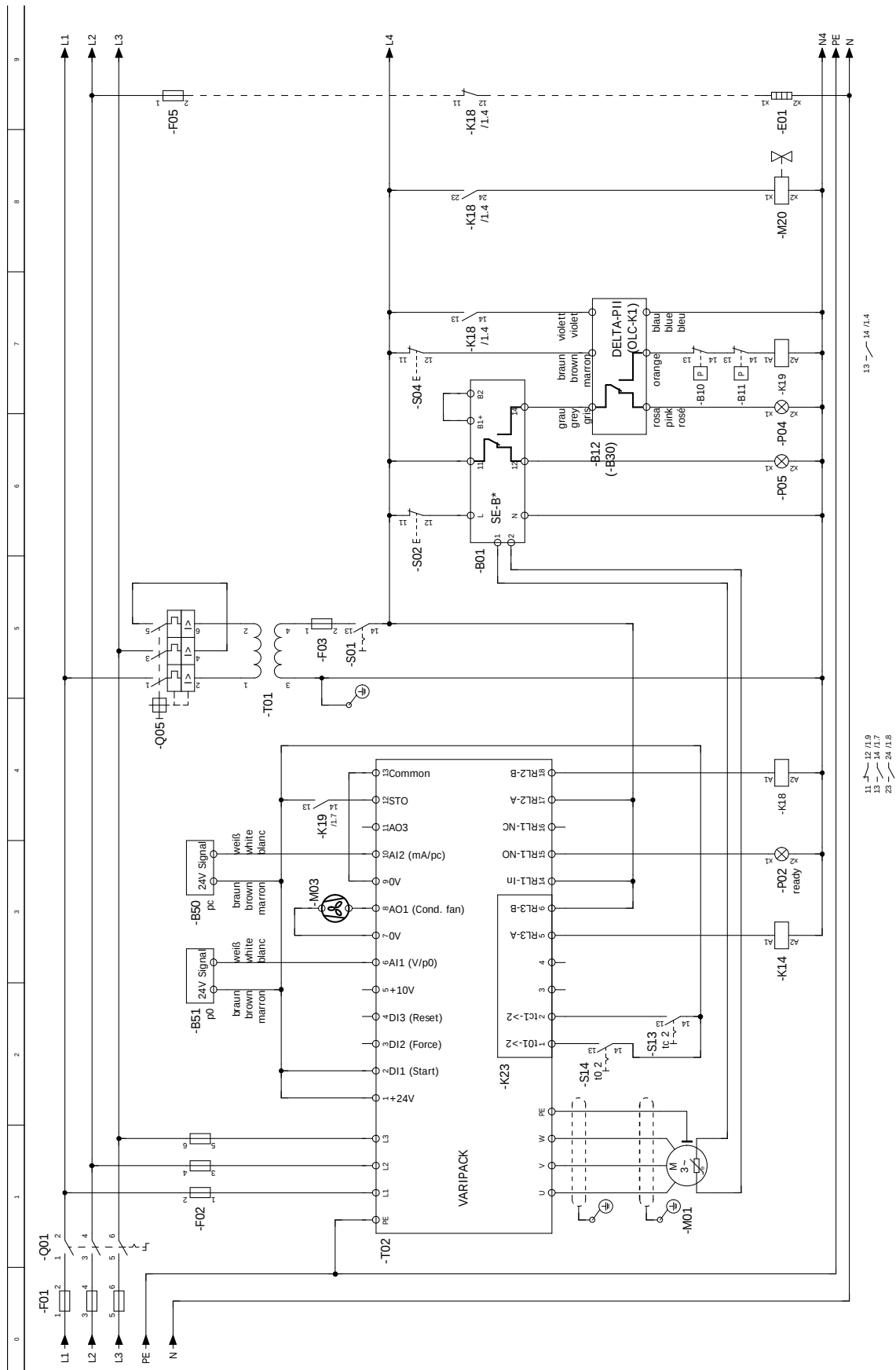
Fig. 13: Schematic wiring diagram of reciprocating compressors with extension module (K23)
